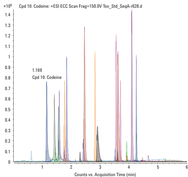
Figure 1. Extracted compound chromatogram of LC/MS Forensic Toxicology Test Mix.
