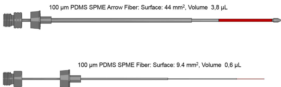
Figure 1. Design of SPME Arrow (above) in comparison with classical SPME (below).
