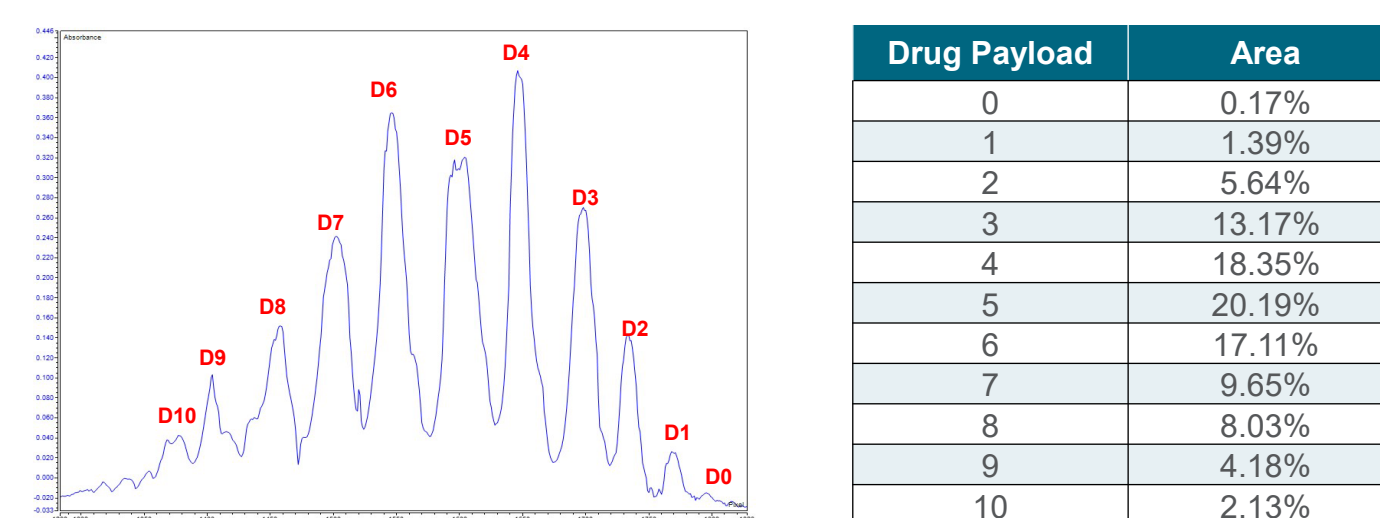
Figure 4. iCIEF-UV profile of T-DM1. About 1.6µg sample was loaded on the column. D0-D10, different drug payloads.
