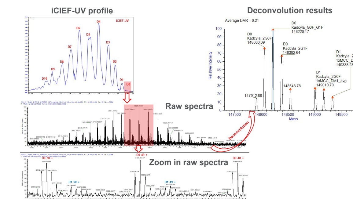
Figure 7. iCIEF-MS spectra and deconvolution results of T-DM1, D0. The complexity of MS spectra was significantly reduced due to iCIEF separation before MS detection.
