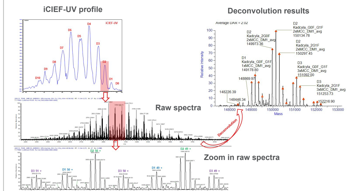
Figure 8. iCIEF-MS spectra and deconvolution results of T-DM1, D2. The complexity of MS spectra was significantly reduced due to iCIEF separation before MS detection.
