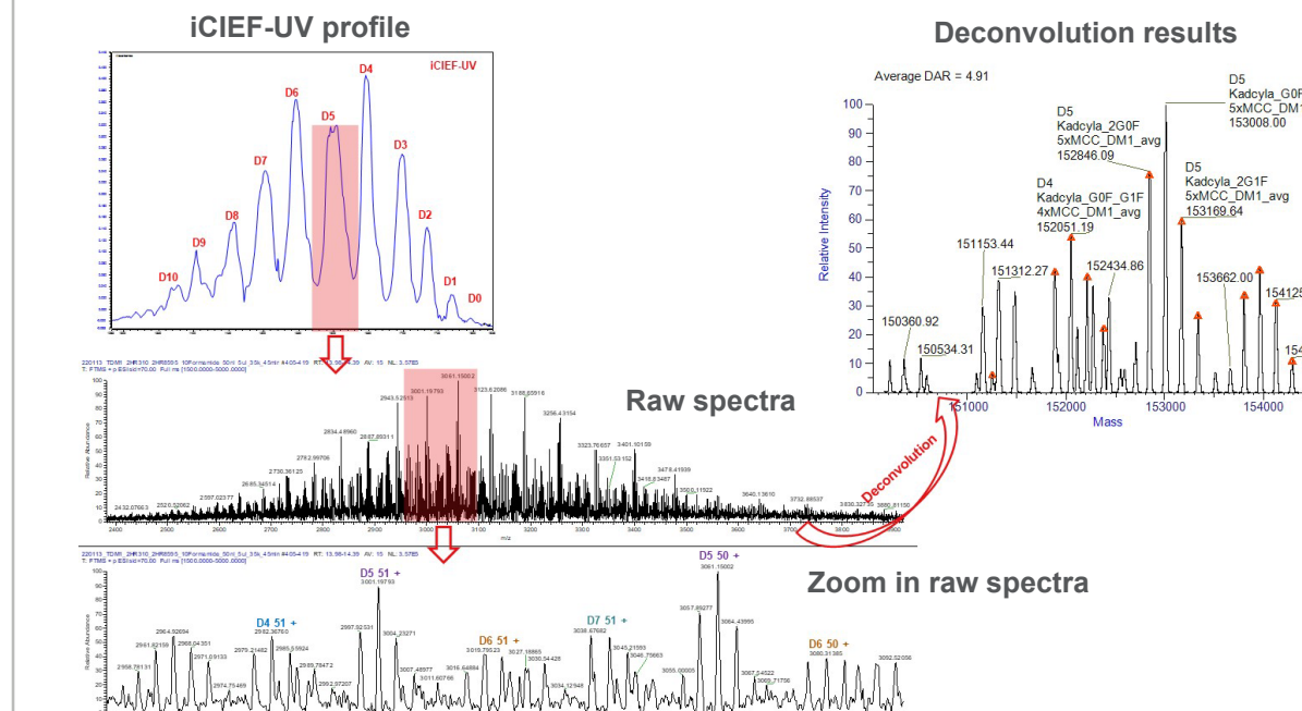
Figure 9. iCIEF-MS spectra and deconvolution results of T-DM1, D5. The complexity of MS spectra was significantly reduced due to iCIEF separation before MS detection.
